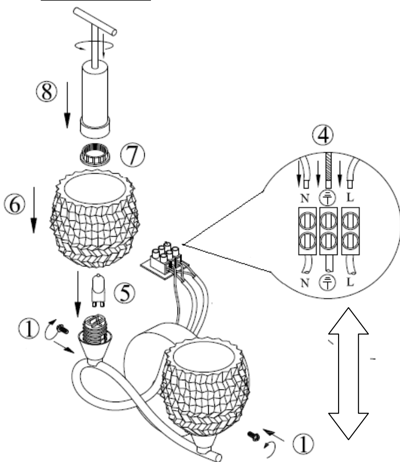
Wiring Details
